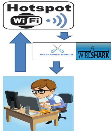
Gambar 3.1 Alur System
