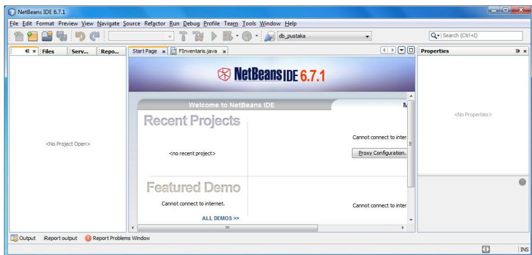
Gambar 1.1 Tampilan netbeans
